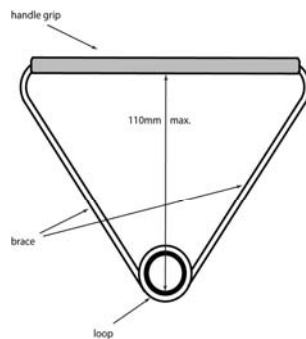
Figure 20 - Generic hammer handle
